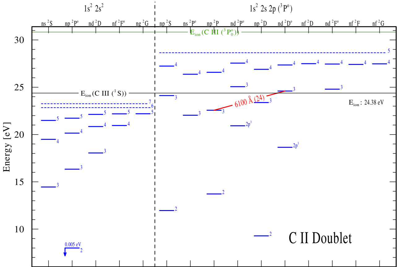
Figure 28: Grotrian diagram adopted from Leuenhagen & Hamann (1994) for C II doublets with 2s^2 singly (left) and 2s\,2p doubly (right) excited states. Triply excited states are indicated by 2p^3 . The levels above the ionization threshold are considered to be in LTE with the C III ground state. None of these LTE levels can auto-ionize (to the C III ground state 2s^2\,^1S ) without radiation, as the inner n = 2 electrons have parallel spins: 1s^2\,2s\,2p(^3P^0) . Therefore, their lifetimes are comparable to normal levels and they can de-excite by a stabilizing line transition, e.g. 2s\,2p\,3d\,^2D^0 - 2s\,2p\,3p\,^2P at 6100\,\text{\AA} .
