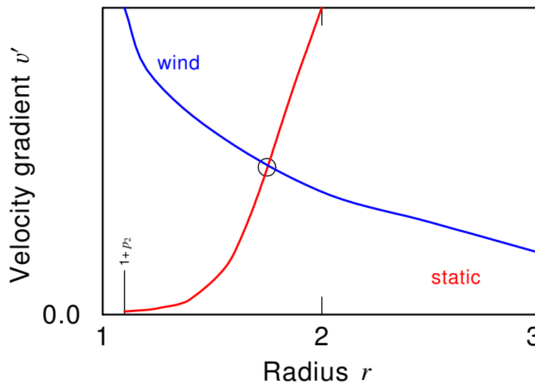
Figure 2: Sketch of the velocity gradient of the hydrostatic law and a beta-law with \beta \leq 1 . In this case, there is certainly one intersection point (encircled).
