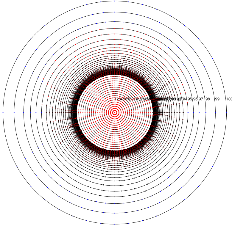
Figure 21: Same as Fig. 20, but in this example the second-model domain is specified as SHAPE=CONE with an inclination angle CONEI=10 and opening half-angle THETA=40 [degrees]. In the cone case with i < \theta (the “hyperbola case”), the red dots mark rays which intersect with the front part of the double-cone, while black crosses denote rays intersecting with the back part; red dots with crosses on top are rays which cut through both parts. Moreover, the calculation includes wind-rotation with VSINI=300 [km/s] which causes additional impact-parameter and angle-points (cf. Fig. 13). For better representation, the wind was cut off beyond 3.0 R_* with NOWIND RADIUS=3.0 as option in FORMAL_CARDS .
