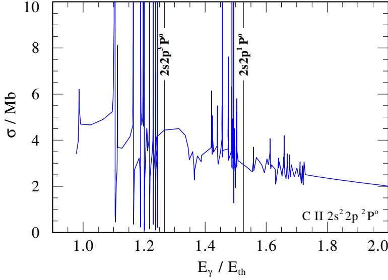
Figure 24: Opacity project photo cross section for C II, summed up over all target states
