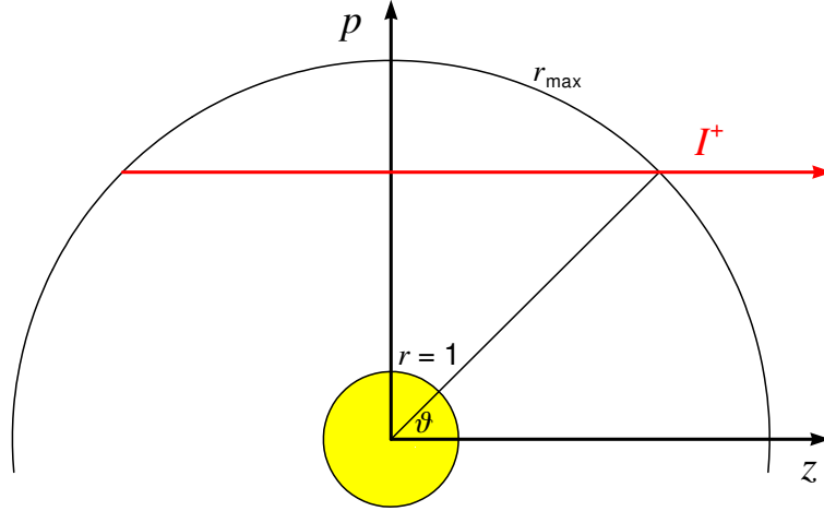
Figure 5: Coordinates are either spherical, with radius r and angle \vartheta , or cartesian with impact parameter p and z in the direction to the observer. The atmosphere is calculated between the inner boundary at r = 1 and the outer boundary at r = R_{\max} .
