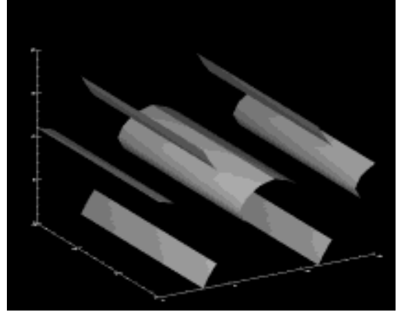
Fig. 1. Convection rolls at \mathcal{R} = 10\,000 without rotation.
