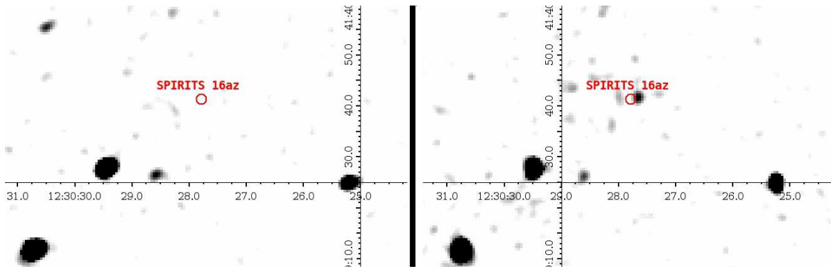
Fig. A.1. Archival not-binned broad-band (0.2–12 keV) X-ray images of NGC 4490 around the position of SPIRITS 16az as indicated by the red circles in each panel. The circle radii are 1'' . The images were obtained by the Chandra ACIS-S camera on 2004-07-29 with an exposure time \sim 39 ks (left panel) and on 2000-11-03 with an exposure time \sim 40 ks (right panel). The X-ray images are shown on linear scale and were smoothed to facilitate perception of the source. North is up, east is to the left.
