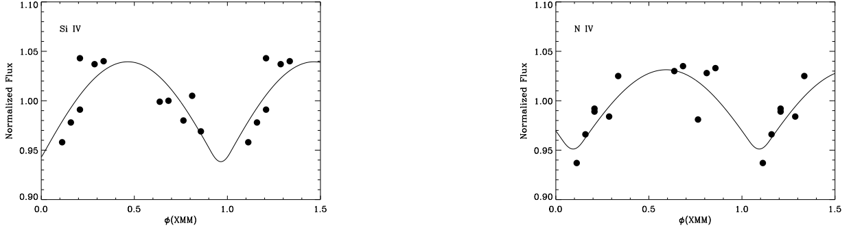
Figure 8. Model fit to the normalized STIS light curves for Si IV \lambda 1402 (left) and N IV \lambda 1718 (right). The parameters for the fits are given in Table 1. The phases are relative to the first XMM-Newton observation.
