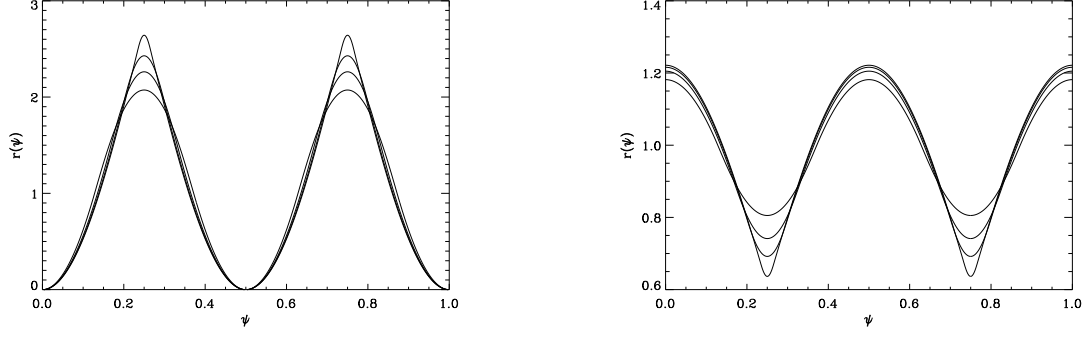
Figure 14. Left: Model light curves for spots that are optically thicker than their surrounding plotted against rotation phase, \psi . The curves are for a_0 = 0.50, 0.25, 0.10 and 0.01 (bottom to top) and were calculated with |C| = 1/a_0 to make them similar over most of their range. Right: Similar curves for the case where the spot is optically thinner than its surroundings. In this case curves with smaller a_0 have the deepest minima.
