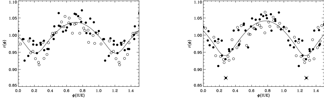
Figure 7. Normalized IUE wind line fluxes for \xi Per binned over -0.2 \leq v/v_\infty \leq 0 for Si iv \lambda 1402 (left) and N iv \lambda 1718 (right) plotted against phase, \phi , relative to the 2.086 day period. Filled circles are for odd phases and open circles are for even phases, which are thought to arise from different spots. The solid curves are fits to the data using eq. (1), resulting in the parameters listed in Table 1. The point in the N iv plot with a cross through it is discordant with its neighbors and was given zero weight in the fit.
