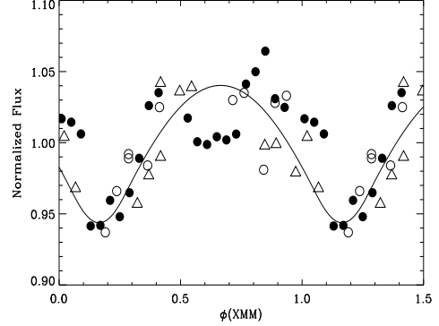
Figure 10. Normalized XMM-Newton and STIS data aligned. Filled circles are for the XMM-Newton fluxes, open circles for the N IV data, and open triangles for the Si IV data. The STIS data have been shifted to align them with the XMM-Newton data to emphasize how they all appear to follow a single period.
