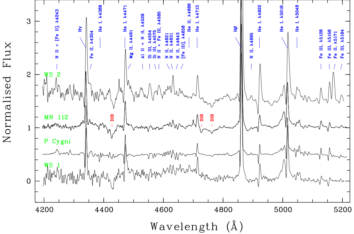
Figure 3. Comparison of normalised blue spectra of WS1 and WS2 with those of the prototype LBV P Cygni and cLBV MN112. The principal lines and most prominent DIBs are identified.
