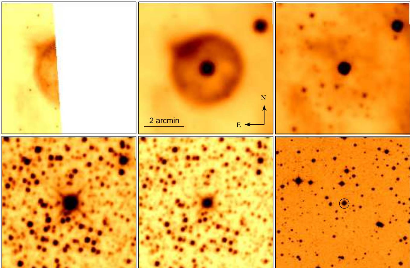
Figure 2. From left to right, and from top to bottom: Spitzer MIPS 24 \mu\text{m} , WISE 22, 12, 4.6 and 3.4 \mu\text{m} and DSS-II red band images of the circular shell WS2 and its central star (marked by a circle on the DSS-II image). The MIPS image is truncated because the MIPS GAL survey covers only a part of the shell. The orientation and the scale of the images are the same.
