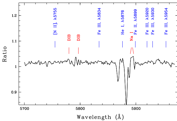
Figure 6. The ratio of the normalised (green) spectra of WS2 obtained within \approx 3 months from each other. The positions of principal lines and most prominent DIBs are indicated.
