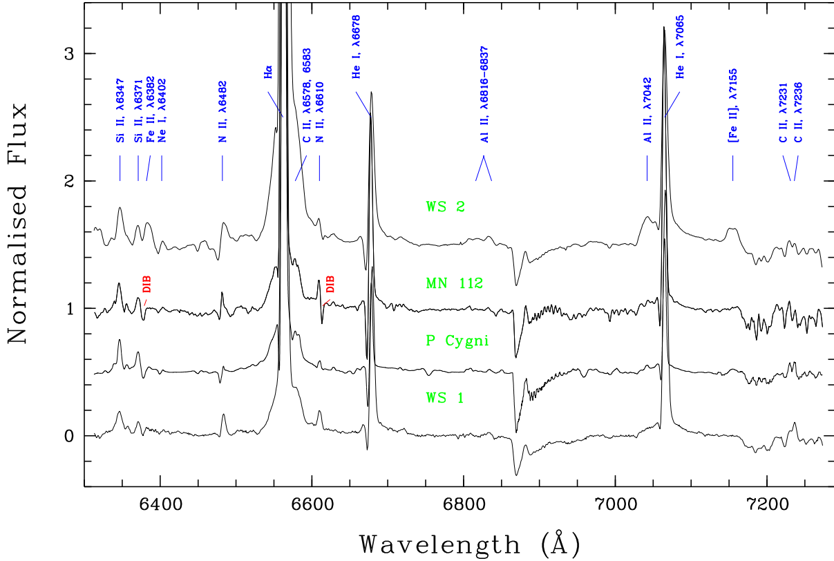
Figure 5. Comparison of normalised red spectra of WS1 and WS2 along with spectra of the prototype LBV P Cygni and cLBV MN112. The principal lines and most prominent DIBs are identified.
