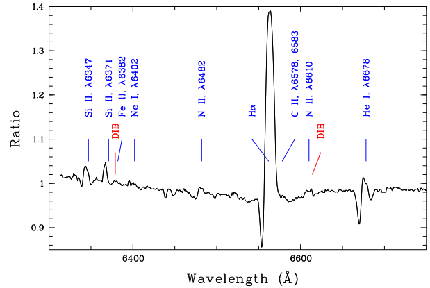
Figure 7. The ratio of the normalised (red) spectra of WS2 obtained within \approx 3 months from each other. The positions of principal lines and most prominent DIBs are indicated.
