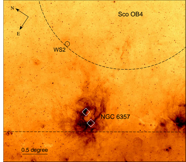
Figure 8. MSX 8.3 \mu\text{m} image of the star-forming region NGC 6357 (containing the star clusters Pismis 24 and AH03 J1725-34.4; indicated by diamonds) and its environments. The position of WS2 is marked by a small circle. The approximate boundary of the Sco OB4 association is shown by a large dashed circle. The Galactic plane is shown by a dashed line.
