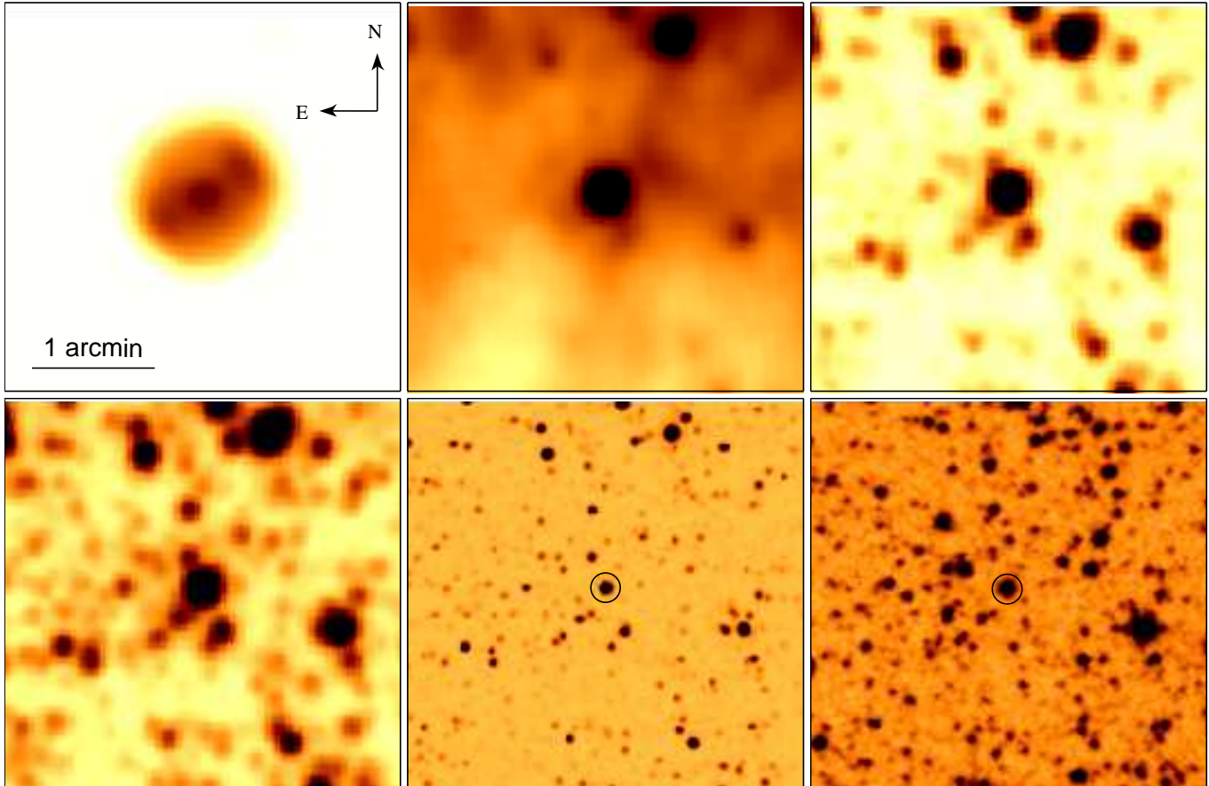
Figure 1. From left to right, and from top to bottom: WISE 22, 12, 4.6 and 3.4 \mu\text{m} , 2MASS K_s -band and DSS-II red band images of the circular shell WS1 and its central star (marked by a circle on the 2MASS and DSS-II images). The orientation and the scale of the images are the same.
