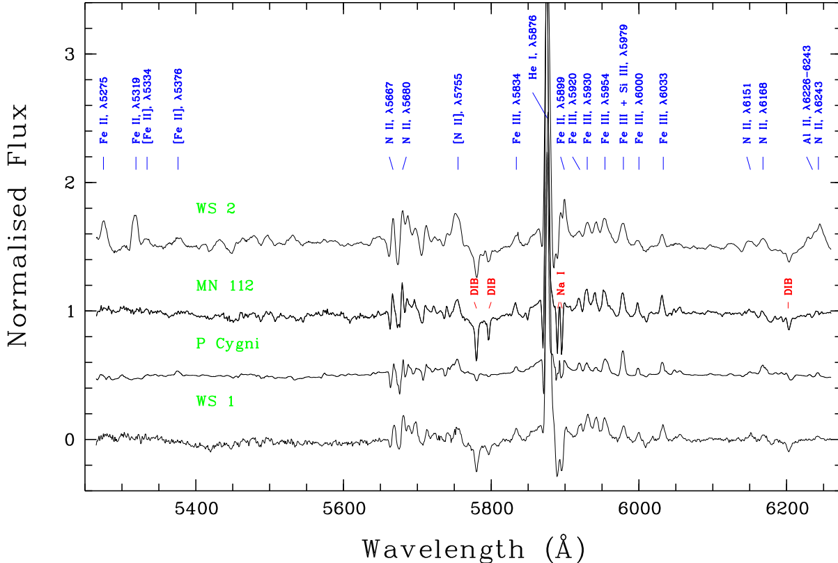
Figure 4. Comparison of normalised green spectra of WS1 and WS2 along with spectra of the prototype LBV P Cygni and cLBV MN112. The principal lines and most prominent DIBs are identified.
