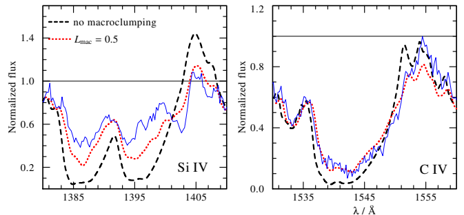
FIG. 10.— The observed Si IV and C IV resonance doublets (left and right panels, respectively) at phase \phi = 0.83 (blue line) compared to the composite synthetic spectrum calculated with the parameters in Table 1, but without macroclumping in the primary (black dashed line), and with macroclumping using L_{\text{mac}} = 0.5 R_* (dotted red line).
