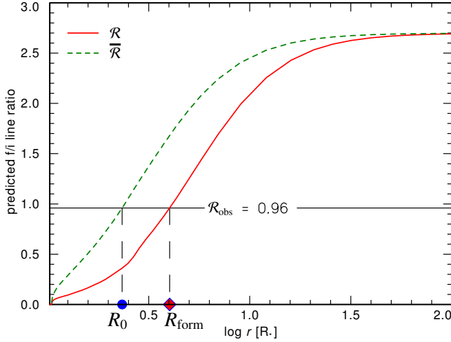
FIG. 13.— Same as Fig. 12, but now accounting for an extended region of X-ray formation (green dashed line). The intersection of \bar{\mathcal{R}}(r) with the observed value delivers the onset radius R_0 .
