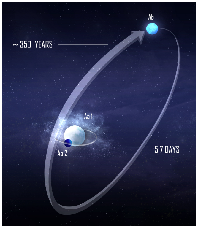
FIG. 1.— Artist's impression of the triple system \delta Ori A, as viewed from Earth. The primary (Aa1) and Secondary (Aa2) form the tight eclipsing binary of period 5.7 d. The primary shows evidence for a significant wind in all spectral domains. A third star (Ab) at an angular separation of \approx 0.3'' ( \sim 100 AU at a distance of d = 380 pc to Earth) orbits the system with a period of \approx 346 yr (Tokovinin et al. 2014) and contributes roughly 25% to the total visual flux. The sizes of all three components are drawn to scale, as inferred in this collaborative study. Their colors reflect their relative temperatures. Note that the tertiary is the second brightest companion in the system. The distance between the binary system Aa and the tertiary Ab is not to scale. Credits to Jessica Mayo
