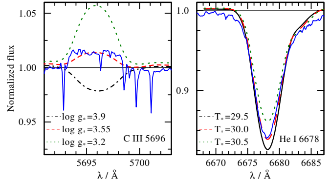
FIG. 8.— Left panel: Sensitivity of C III \lambda 5696 to gravity. The observed spectrum at phase \phi = 0.02 (blue line) is compared to three composite synthetic spectra calculated with the parameters given in Table 1, but with \log g_* of the primary set to 3.9, 3.55, and 3.2 (black dotted-dashed, red dashed, and green dotted lines, respectively). Right panel: Sensitivity of He I \lambda 6678 to temperature. We set the temperature of the primary to 29.5, 30.0, and 30.5 kK (black dotted-dashed, red dashed, and green dotted lines, respectively).
