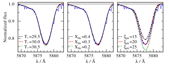
FIG. 6.— Sensitivity of the He I \lambda 5876 line to temperature, helium abundance, and microturbulence. The observed spectrum (blue line) at phase \phi = 0.84 is plotted along with three composite synthetic spectra calculated with the parameters given in Table 1, but with different temperature (left panel: T = 29.5, 30, 30.5 \text{ kK} ), helium abundance (middle panel: X_{\text{He}} = 0.2, 0.3, 0.4 ), and photospheric microturbulence (right panel: \xi_{\text{ph}} = 15, 20, 25 \text{ km s}^{-1} ) for the primary model (black dotted-dashed, red dashed, and green dotted lines, respectively).
