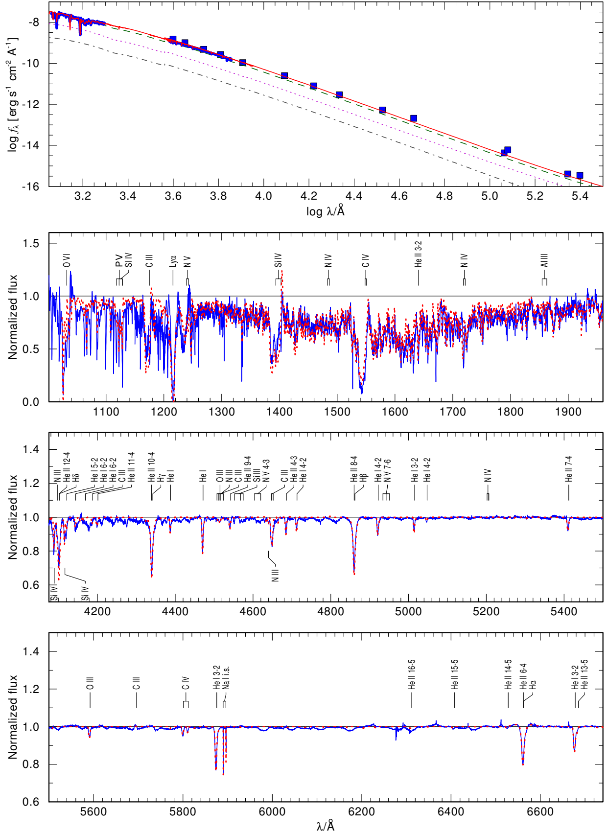
FIG. 2.— Upper panel: Comparison between observations (blue squares and lines) and the total synthetic SED (red solid line), which consists of the primary (green dashed line), secondary (gray dash-dotted line), and tertiary (pink dotted line) models. Lower panels: Comparison between the composite synthetic (red dotted line) and observed (blue line) normalized spectra in the UV and optical. Both spectra roughly correspond to phase \phi = 0.54 . For clarity, we refrain from showing the contributions of each component model to the normalized spectrum. The wavy pattern seen in the observed spectrum (e.g., in \approx 6000 - 6200 Å) is an artifact caused by connecting the echelle orders, not related to the stellar system.
