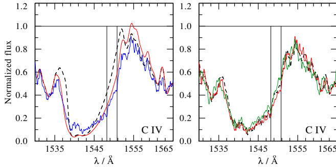
FIG. 7.— Left panel: observed C IV resonance doublet at phase \phi = 0.73 (blue line) is compared to two synthetic composite spectra, with increased wind turbulence of \xi_w = 200 \text{ km s}^{-1} in the primary model (red solid line), and without it (black dashed line). Large microturbulent velocities beyond the sonic point are the only mechanism that can reproduce the redshifted absorption trough. Note that a further improvement of the profile is achieved by accounting for macroclumps, which are not included here. Right panel: Comparison of three IUE observations at phases \phi = 0.18, 0.73, 0.98 (black, red, and green lines, respectively), illustrating that the redshifted absorption trough is observed at all phases.
