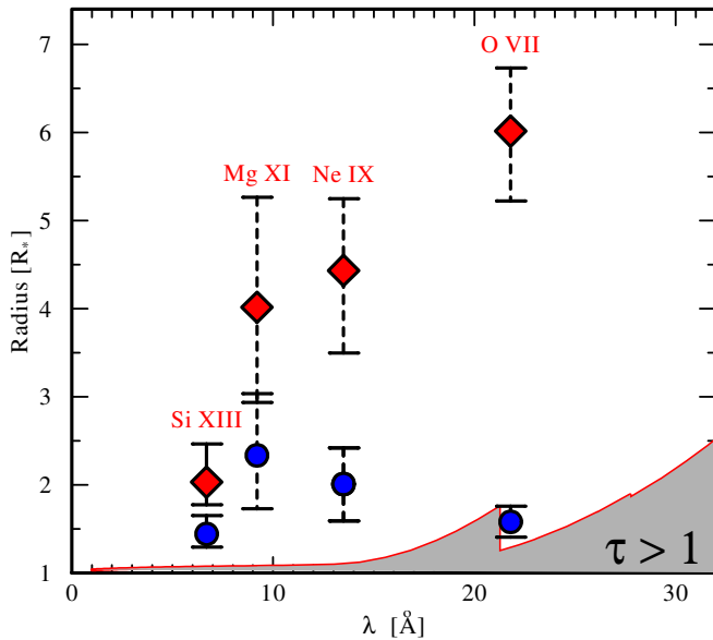
FIG. 14.— Inferred formation radii (red diamonds) and onset radii (blue circles) of the X-ray radiation, as inferred from the four He-like ions Si XIII, Mg XI, Ne IX, and O VII. The error bars correspond to measurement uncertainties propagated into errors of the inferred radii (see Fig. 13). The shaded area corresponds to radii at which \tau_{\text{Ross}} \geq 1 .
