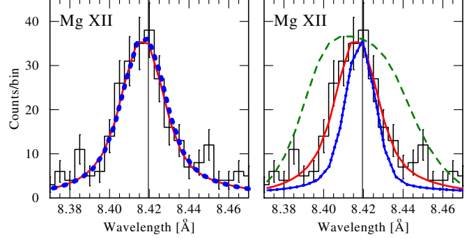
FIG. 15.— Left panel: Observed co-added HEG \pm 1 spectrum of \delta Ori A centered on the Mg XII line (histogram), compared with a smooth-wind model (blue dotted line), and a clumped model (red solid line). As anticipated, clumping hardly affects the line formation at short wavelengths. Right panel: Again Mg XII, with three smooth models which assume X-ray onset radii of 1.01 R_* (blue dotted-solid line), 1.1 R_* (red solid line) and 1.5 R_* (green dashed line), suggesting that X-ray radiation initiates roughly at 1.1 R_* (for the adopted velocity law). The vertical lines indicate the rest wavelength shifted with the systemic velocity 15 \text{ km s}^{-1} .
