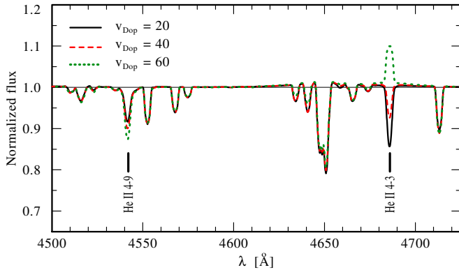
FIG. 5.— This figure illustrates the extreme sensitivity of the He II \lambda 4686 line to the parameter v_{\text{Dop}} . Here we depict only the primary model, calculated with the parameters in Table 1, but with v_{\text{Dop}} = 20 \text{ km s}^{-1} (black solid line), 40 \text{ km s}^{-1} (red dashed line), and 60 \text{ km s}^{-1} (green dotted line). The formal integration is performed with the same turbulent velocity as given in Table 1. Notice that most lines hardly react to this parameter.
