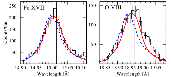
FIG. 16.— Left panel: Observed co-added MEG \pm 1 spectrum of \delta Ori A centered on Fe XVII line (histogram) and two wind model lines: smooth (blue dotted line) and clumped (red solid line). The onset of X-ray emitting plasma is at 1.2 R_* . Right panel: Same as left panel, but for the O VIII line.
