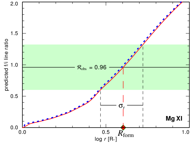
FIG. 12.— Theoretical f/i ratio \mathcal{R}(r) is plotted as a function of the X-ray formation radius (blue dotted line) for the Mg XI ion. The intersection of \mathcal{R}(r) with the observed value \mathcal{R}_{\text{obs}} implies the formation radius under the assumptions of the point-like approach. The error \sigma_r in the formation radius corresponds to 1-\sigma measurement uncertainties in \mathcal{R}_{\text{obs}} , depicted by the green shaded rectangle. The red solid line depicts \mathcal{R}(r) as well, but includes the contribution of collisions assuming a full ionization and a factor 1000 density enhancement in the shocked plasma
