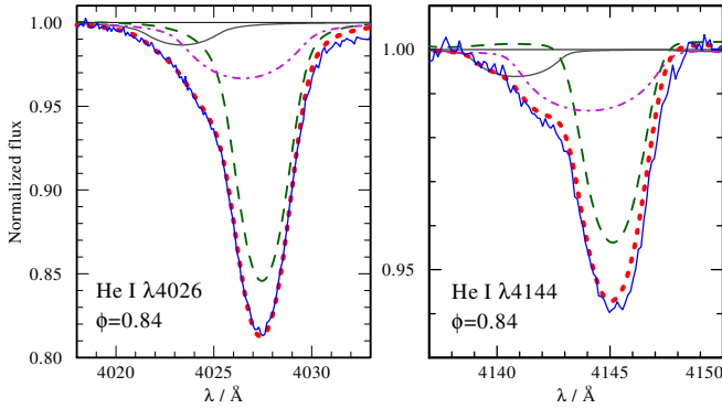
FIG. 4.— The two panels depict two observed He I lines (blue lines) at phase \phi = 0.84 in which the secondary may be detectable. The different curves correspond to the primary (green dashed line), secondary (gray solid line), tertiary (pink dashed-dotted line), and total (red dotted line) synthetic spectra.
