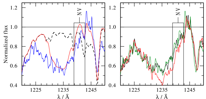
FIG. 11.— Left panel: Observed N V resonance doublet at phase \phi \sim 0.1 (blue line) with two synthetic composite spectra, calculated with the parameters in Table 1, not including X-rays (black dashed line), and including X-rays (red solid line). Right panel: Like the right panel of Fig. 7, the three IUE observations at phases \phi = 0.8, 0.3, 0.1 (black, red, and green lines, respectively).
