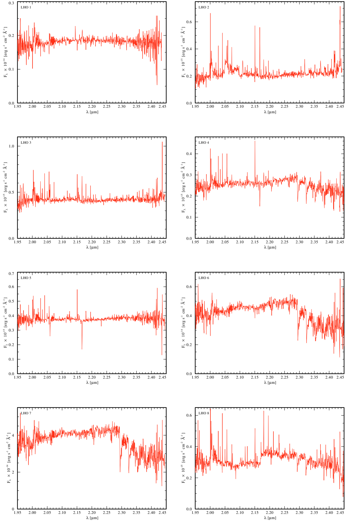
Fig. 11. Spectral atlas, spectra are rebinned with 4 \text{ \AA} .
