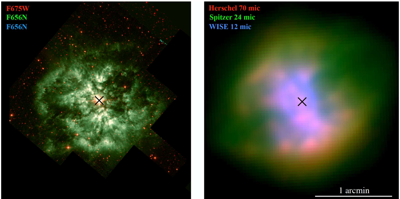
Figure 1. Color-composite pictures of M1-67. Left: HST image. Right: IR image. The position of WR124 is shown with a cross in the two panels. Both images have the same field of view. North is up and east to the left.
