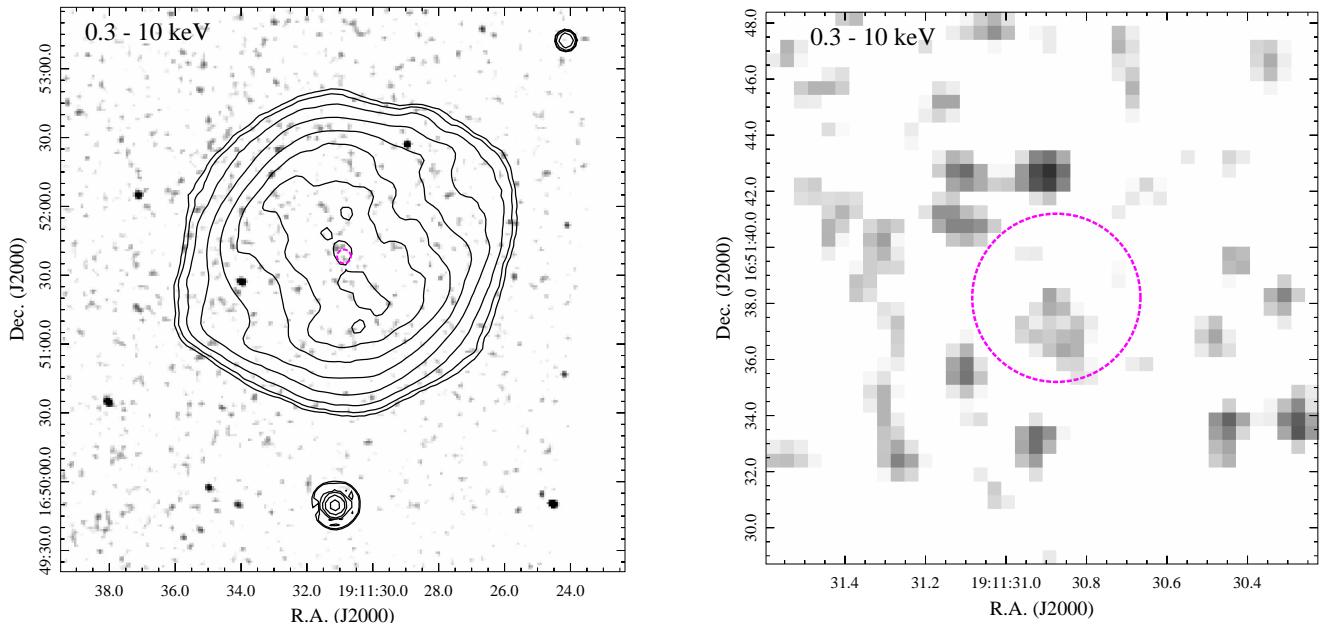
Figure 2. Left: Chandra ACIS-S X-ray image of the field of view around WR 124 in the 0.3–10 keV energy range and combining all four observations. The contours show the 24\ \mu\text{m} emission as detected by Spitzer MIPS (see Fig. 1). Right: Same as left panel but smaller field of view around WR 124. The magenta circle in both panels is centered at the position of WR 124 with an angular radius of 3'' .
