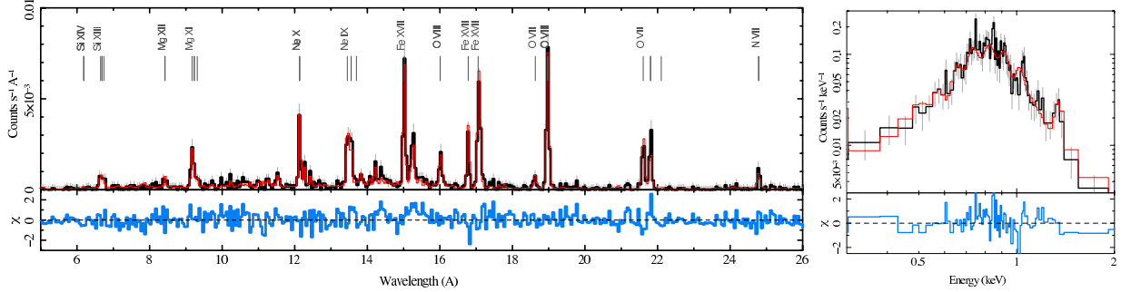
Fig. 1.— \mu Col Chandra /LETG/ACIS spectrum (left); black: observed count-rate; thin-gray line (red in the online version): model; the lower panel shows the \chi^2 residuals against a broken power-law APEC model modified for photoexcitation of triplets. Lines are broader than the instrumental width. The Suzaku spectrum is shown on the right (black). For conciseness, we have summed the counts from the three detectors; such is not recommended when fitting, but it provides a good summary visualization of the data. The folded Chandra -derived model is in gray (red in the online version), and residuals below. We emphasize that the Chandra -derived model was not fit to the Suzaku spectrum, only folded through the response to provide model counts and residuals; the model agrees very well without any adjustments. It is significant that there is little or no flux detected above 2 keV where Suzaku has substantial sensitivity.
