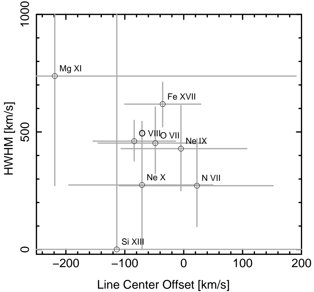
Fig. 3.— \mu Col emission line Doppler offset and width; errorbars give 90% confidence limits. Due to lower resolution at shorter wavelengths, the Mg XI and Si XIII lines are poorly constrained. The systemic line-of-sight velocity of 109.2 \text{ km s}^{-1} (Evans 1967) has been removed.
