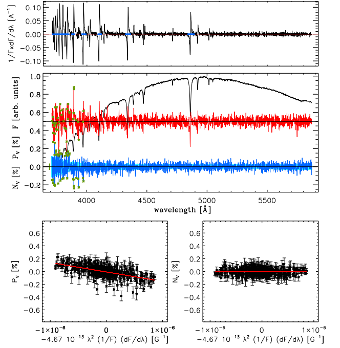
Fig. 1. Graphical output of the IRAF/IDL “Bonn pipeline” obtained from the analysis of the FORS 2 data of HD 23478 considering the hydrogen lines. The top panel presents the derivative of Stokes I . The regions used for the calculation of the magnetic field are marked by a thick blue line centered at zero. In the middle panel, the top spectrum presents the Stokes I spectrum arbitrarily normalised to the highest value, the middle red spectrum corresponds to the Stokes V spectrum (in %), while the bottom blue spectrum is the N spectrum (in %). The green asterisks drawn on the Stokes V and N spectra mark the points which have been removed by the sigma clipping. The pale blue strip drawn behind the N spectrum shows the uncertainty associated with each spectral point. As a double-check of the statistical consistency of the data and uncertainties, the thick green bar on the left side of the N spectrum shows the standard deviation of the N profile. In the bottom-left panel, we present the linear fit used for the determination of the magnetic field value using Stokes V (i.e. \langle B_z \rangle ). The red solid line shows the best fit. From the linear fit we obtain \langle B_z \rangle = -1477 \pm 95 \text{ G} . In the bottom-right panel, we present the same as in the bottom-left panel, but for the null profile (i.e. \langle N_z \rangle ). From the linear fit, we obtain \langle N_z \rangle = 30 \pm 64 \text{ G} .
