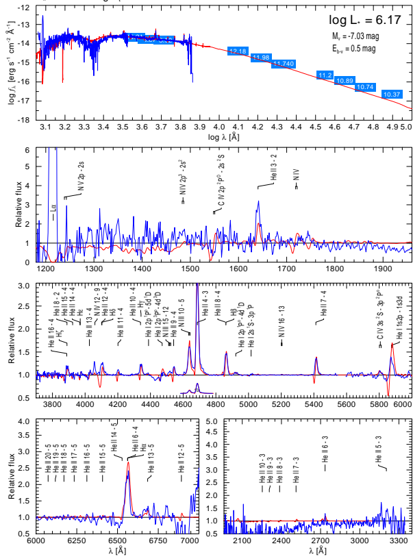
Fig. C.32. Spectral fit for BAT99 079 and BAT99 080
