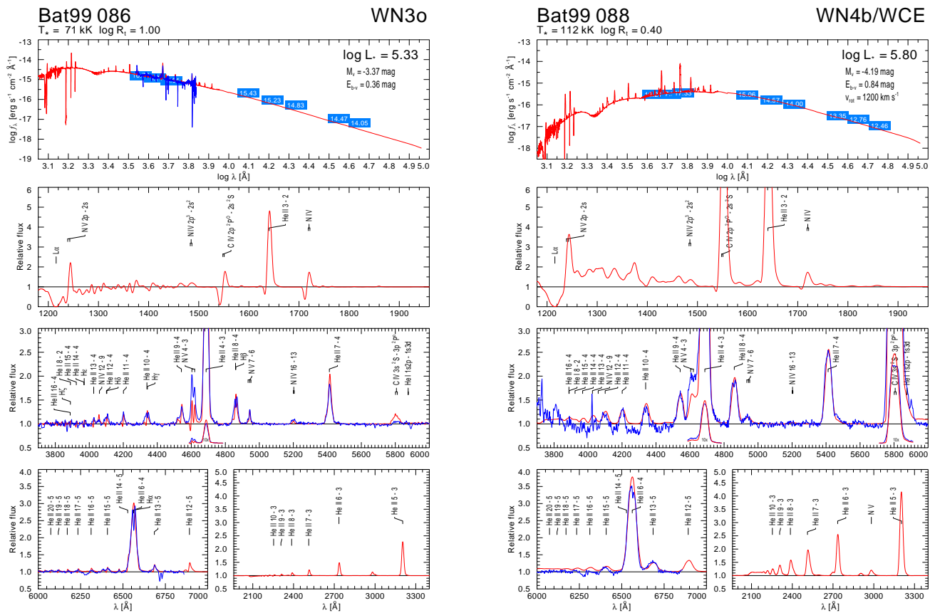
Fig. C.34. Spectral fit for BAT99 086 and BAT99 088
