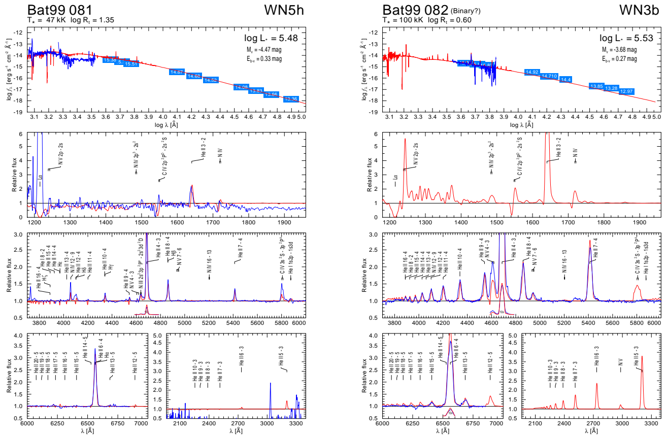
Fig. C.33. Spectral fit for BAT99 081 and BAT99 082
