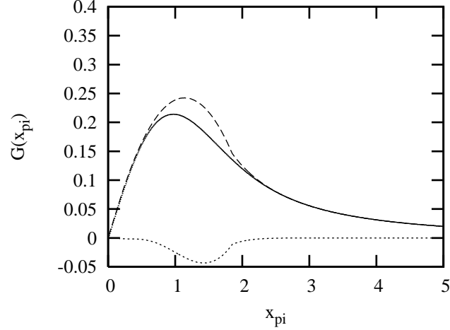
Figure 1. The plot of the Chandrasekhar function. The exact function G(x) according to (11) is plotted by a solid line, the approximation G_A(x) after (16) by a dashed line, and the difference between both G(x) - G_A(x) by a dotted line.
