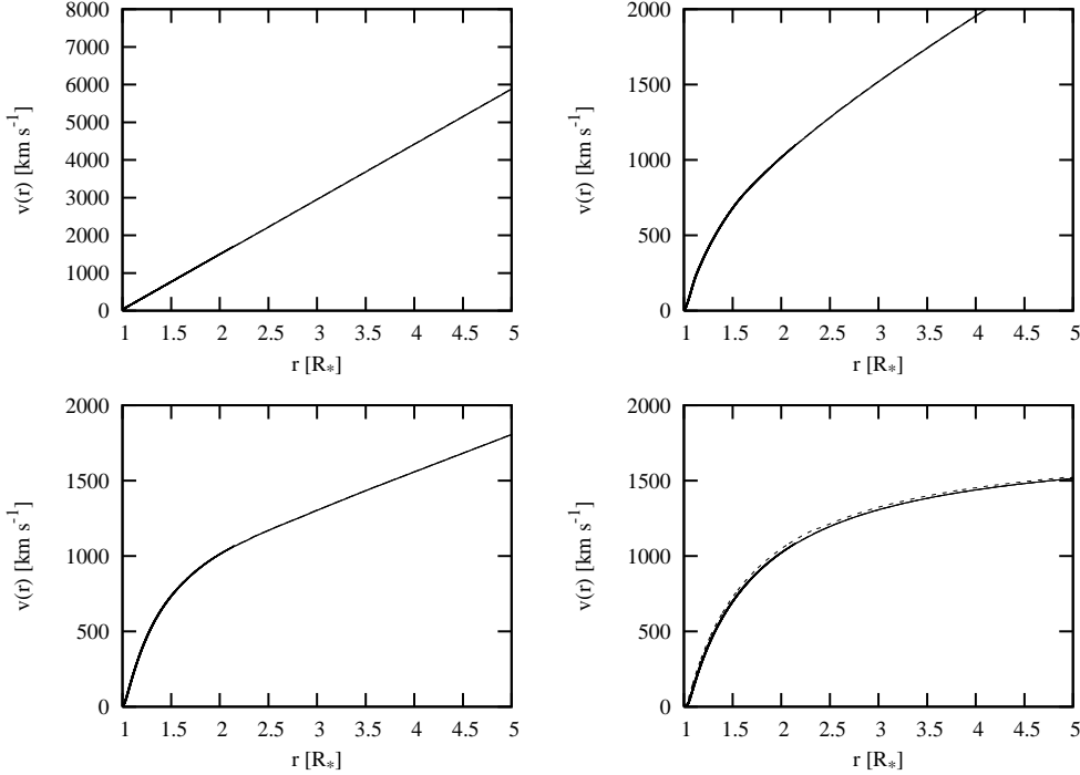
Figure 2. Upper left panel: The initial condition of velocity for a time dependent two-component model of a \tau Sco star from Table 1. This star was chosen due to its predicted well coupled stellar wind. Upper right panel: After few time steps we can see, how the velocity profile is attracted to the CAK solution. Lower left panel: The same situation but much later and closer to the CAK solution. Lower right panel: Finally, it converged to the CAK type solution. We compared our two-component model with a one-component simulation. We see that the two-component solution (dashed line) corresponds with the one component solution (solid line).
