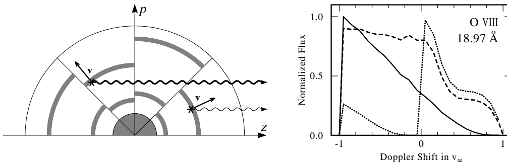
Figure 1. Left panel: Sketch of the blob-shell collision model. Optically thick material is fragmented in radial shells expanding with constant velocity \mathbf{v} . The vicinity of the star inside the radius R_{\text{inner}} , where the fragmentation occurs, is filled with homogeneous material moving with v \propto r (grey circle). The thick black line indicates the path along which photons move towards the observer without being intersected by a shell. The thin black line indicates the path of photons which suffered absorption. Right panel: Line profiles of O VIII for the parameters of \zeta Pup (Puls et al. 1998). The full-drawn line represents the case when the wind is homogeneous. The dashed line represents Case I. The opacity is reduced only for the photons originated in the red part of the line, but those in the blue part are severely depleted by absorption in the natal shell. The dotted line represents Case II. The opacity is reduced and the line is more centered, compared to the homogeneous case. This case resembles most the observed line profile (Cassinelli et al. 2001). The shoulder in the red part of the lines is due to the absorption by the homogeneous inner wind.
