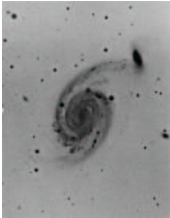
Figure 17: NGC 7753/2.
