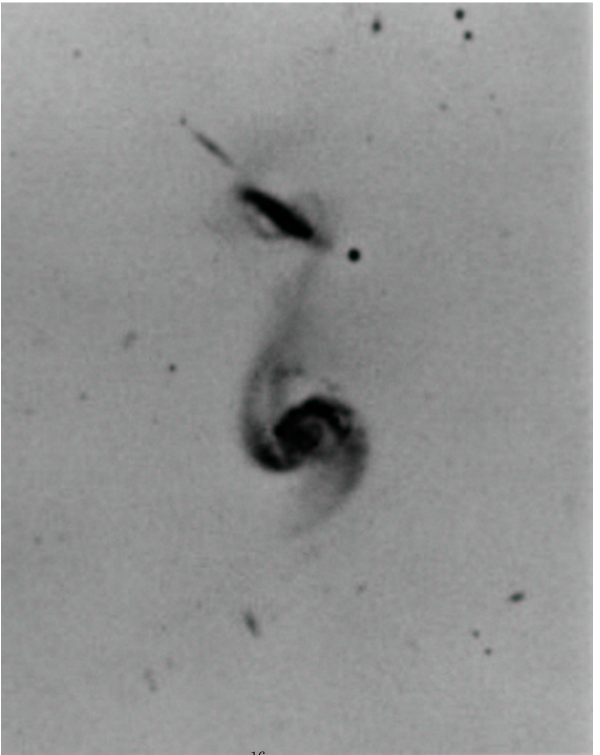
Figure 16: Bridges (NGC 3808).
