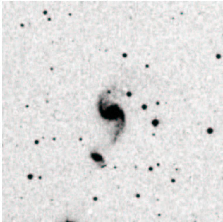
Figure 15: Bridges (NGC2535/6).
