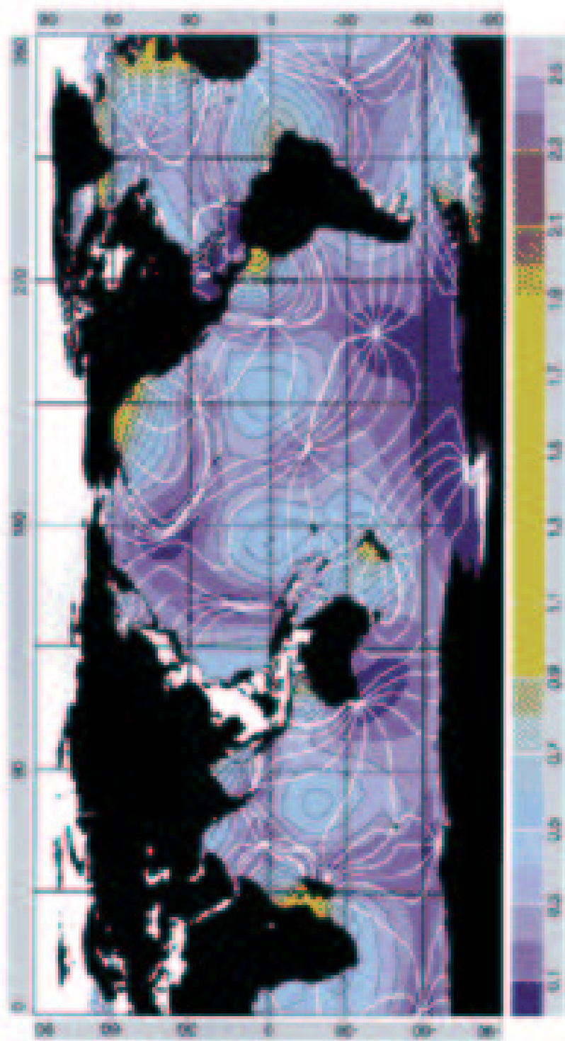
Figure 8: Satellite 8 data of cotidal lines.
