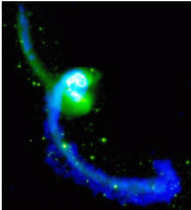
Figure 21: Tails (NGC4038/9, the Antenna).
