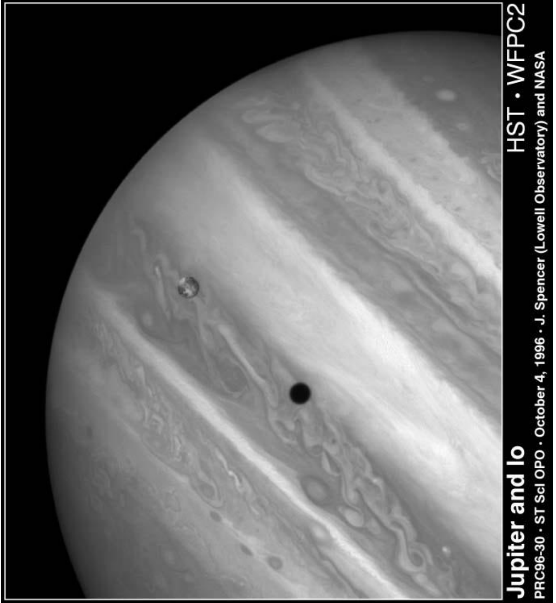
Figure 9: Jupiter and Io.
