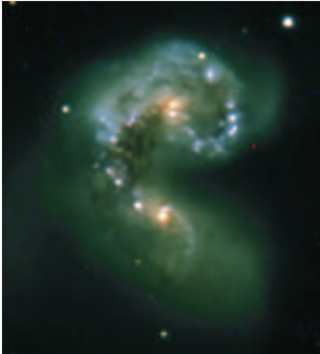
Figure 20: Tails (NGC4038/9, the Antenna).
