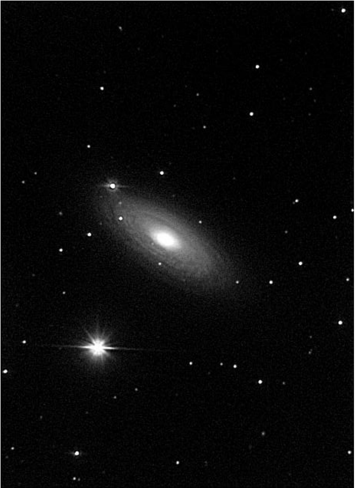
Figure 23: Flocculent galaxy (NGC2841).
