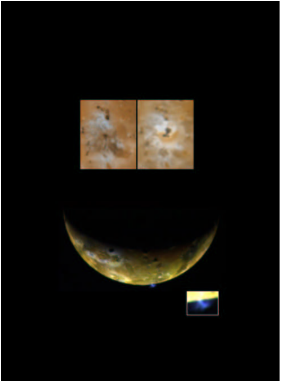
Figure 10: Image taken by Galileo spacecraft with 100 km high volcano eruption.
