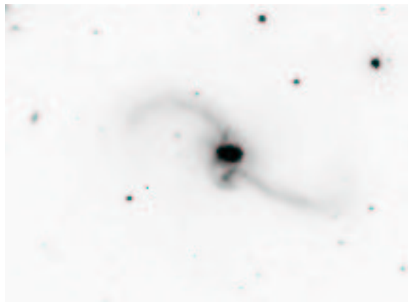
Figure 19: Tails (NGC2623).
