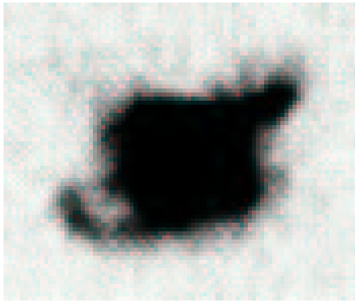
Figure 22: Quasar 3CR 249.1 at z=0.31 (Stockton & MacKenty 1987).
