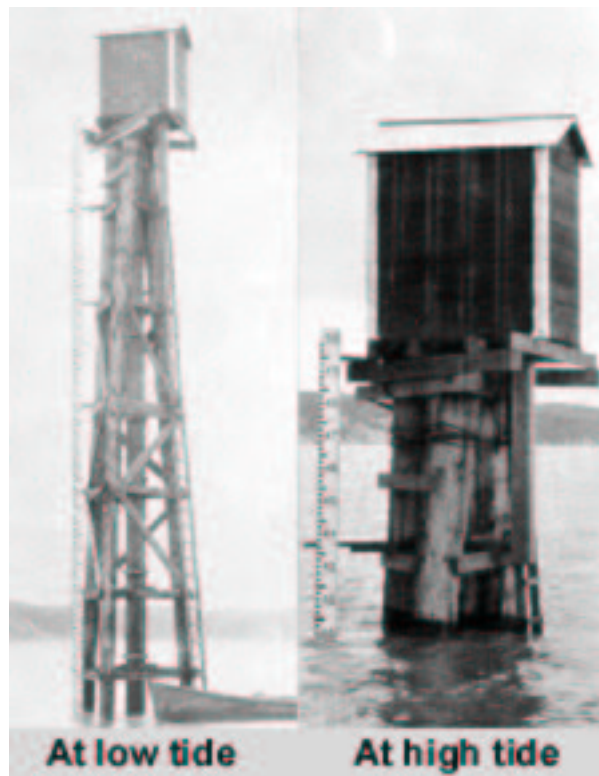
Figure 2: Tides in Anchorage.
